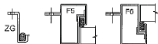
Flange Mounted Integral Gasket Frames ( for Fume tight & Weather tight )
